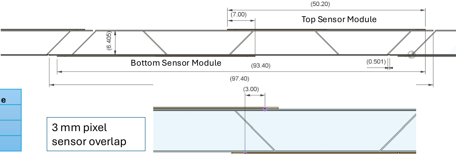
2x Forward disks (A and C side)
