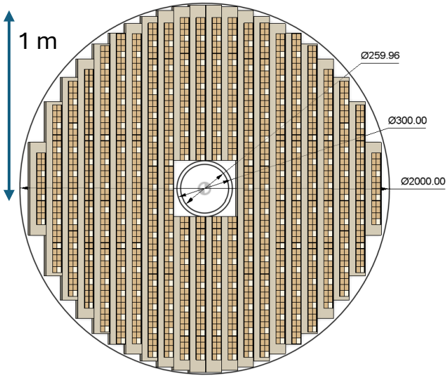
2x Forward disks (A and C side)
