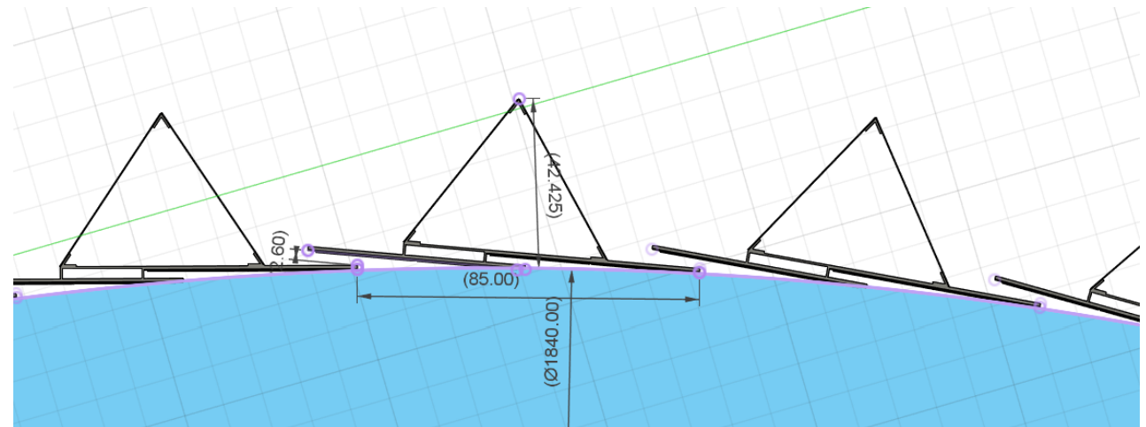
C Side Half Stave Layout
